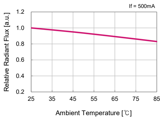
▪ Ambient Temperature vs. Relative Radiant Flux
