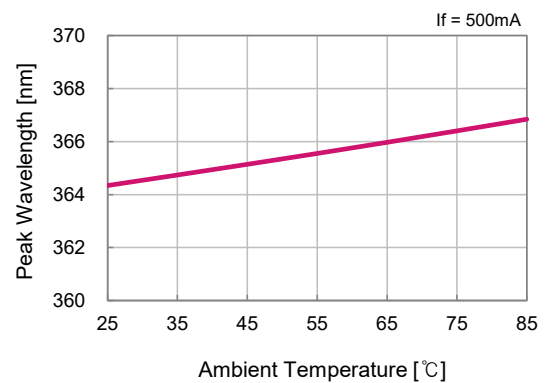
▪ Ambient Temperature vs. Peak Wavelength
