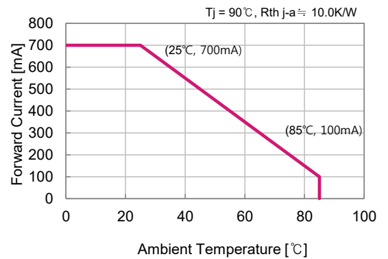
▪ Derating Curve
