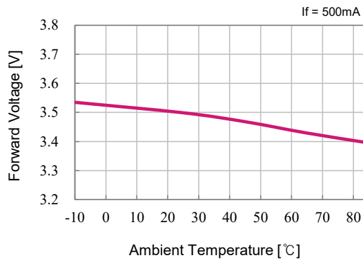
▪ Ambient Temperature vs. Forward Voltage
